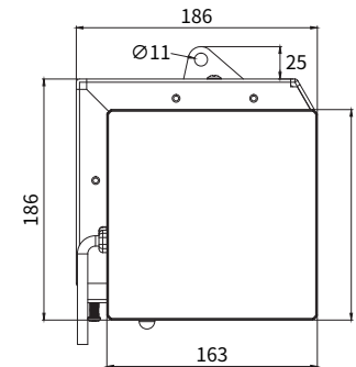
Side view of the casing
